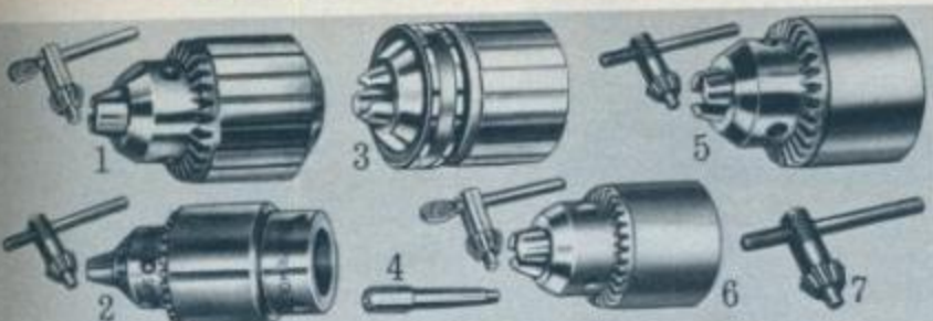
1 Geared Key Headstock Chucks. Key type. Key included.
